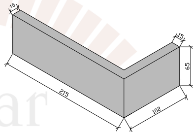
Corner Brick Slip
