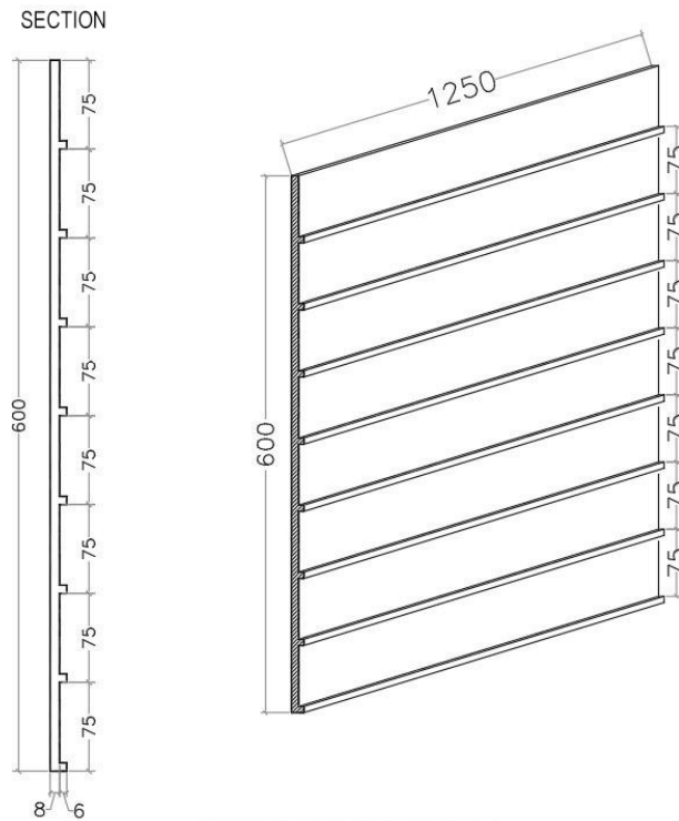
CHANNELED GRC BOARD PANEL
